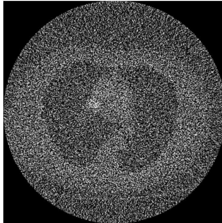
shepp-logan RMSE=0.00052 | PSNR=5.76 dB | SSIM=0.18449
