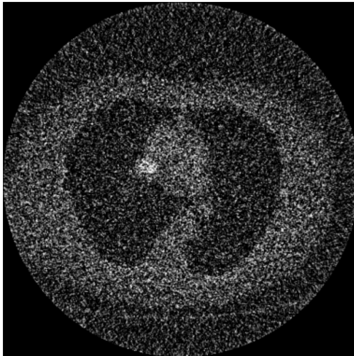
SIRT (200 iter) RMSE=0.00021 | PSNR=13.39 dB | SSIM=0.20156
