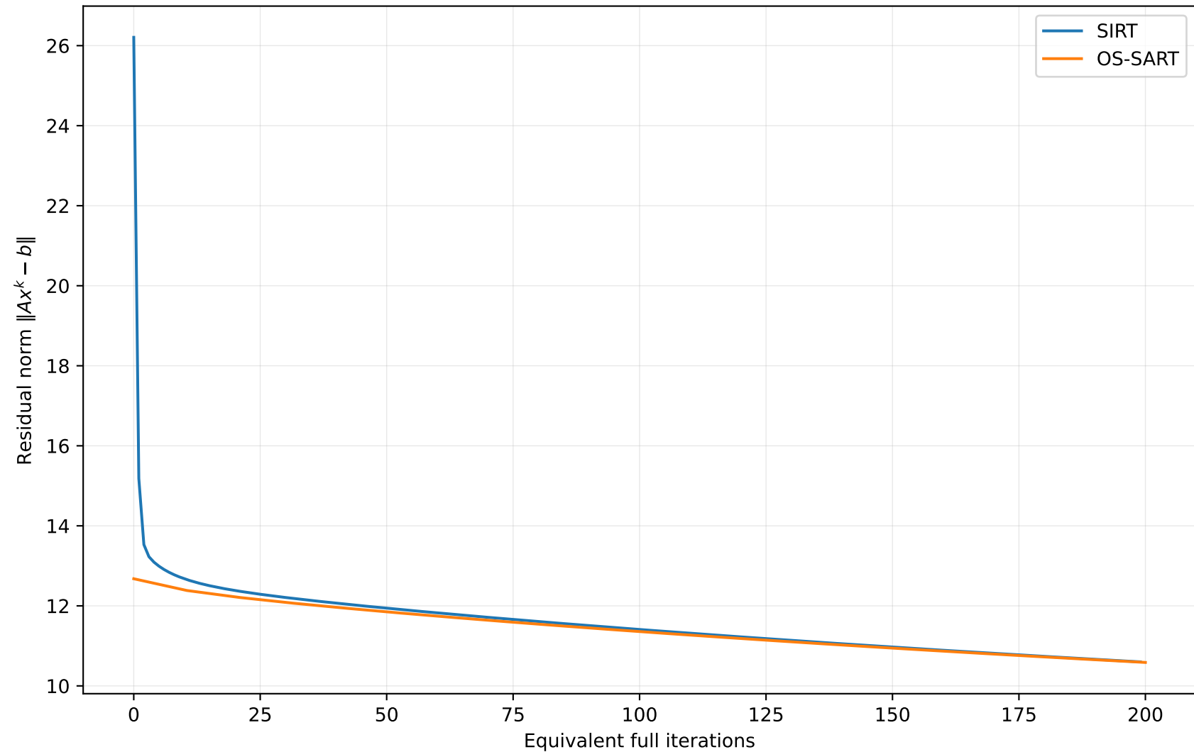
Figure 1.3c: SIRT vs OS-SART Convergence
