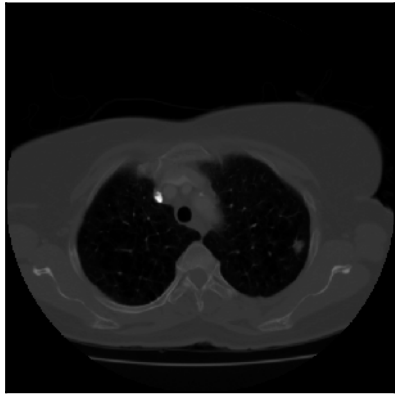
GT
