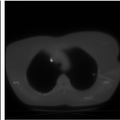
Fixed PnP-ADMM
