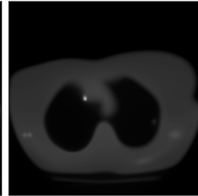
TFPnP
