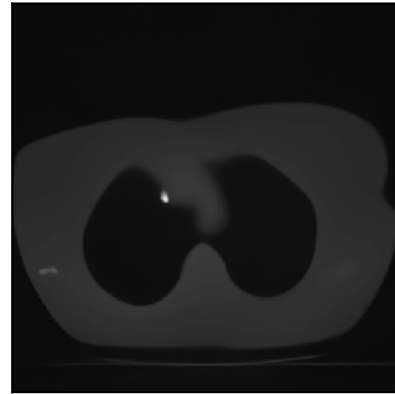
DRUNet
