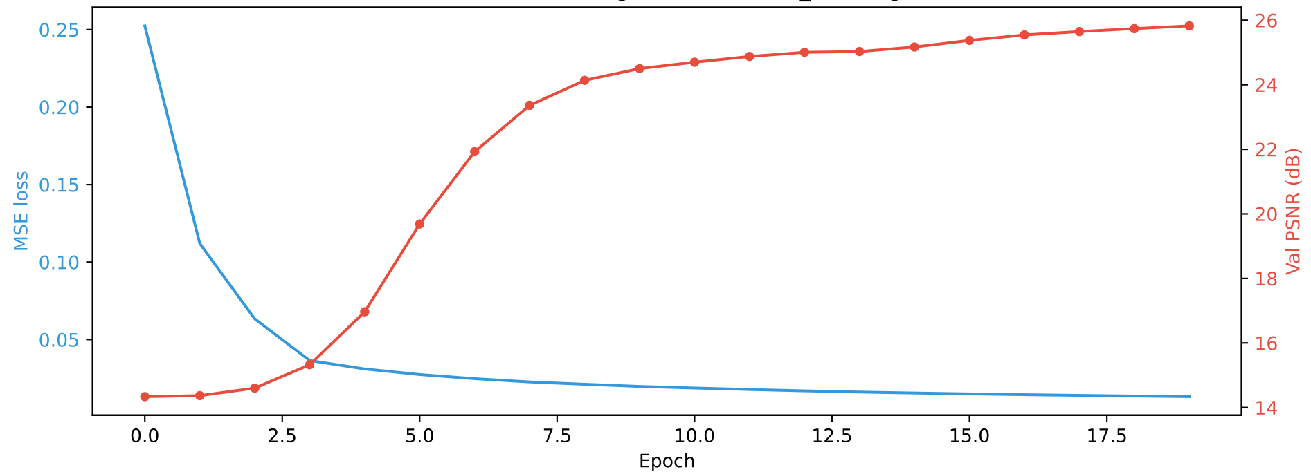
FBPConvNet training (250 × 80, run_04 budget)
