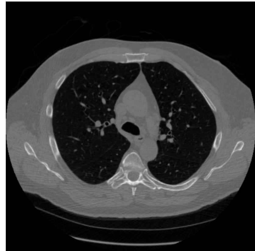
Ground truth
