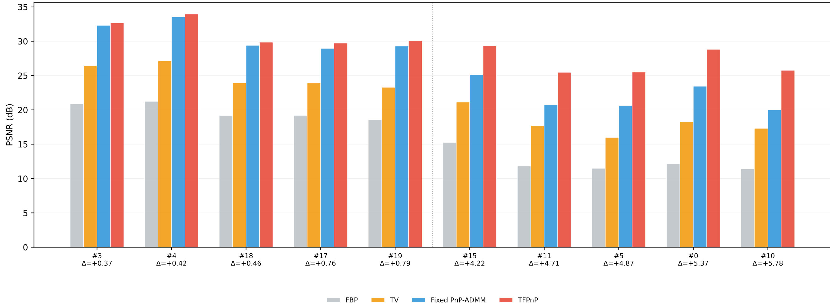
Per-Image PSNR at 5% Noise — 5 smallest and 5 largest TFPnP-Fixed PnP gaps
