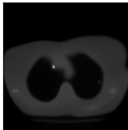
TFPnP
