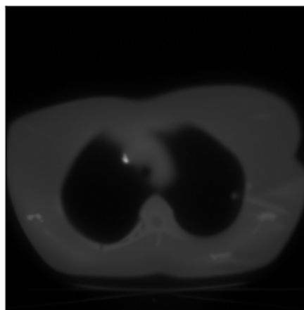
Fixed PnP-ADMM
