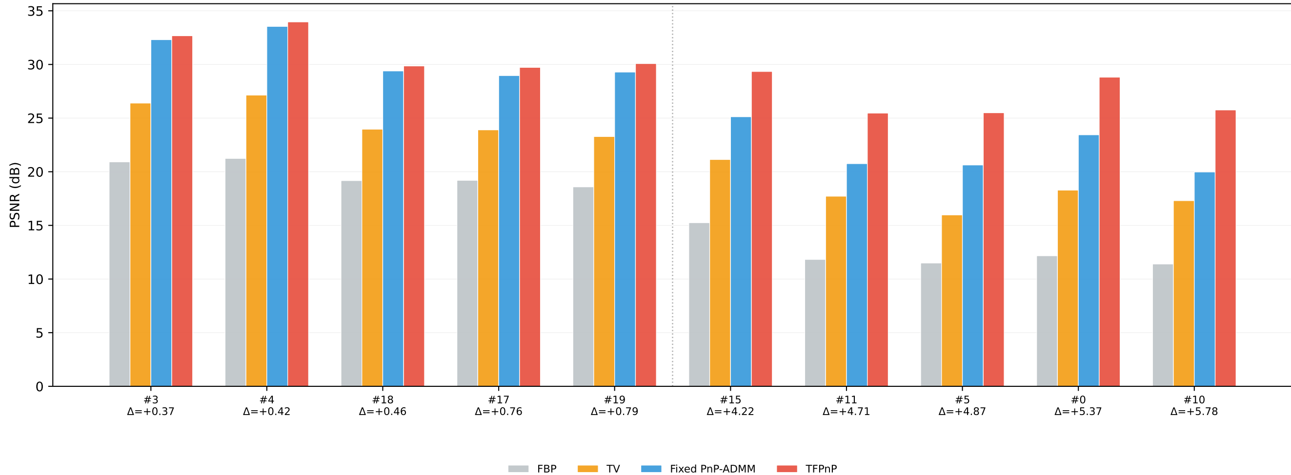
Per-Image PSNR at 5.0% Noise — 5 smallest and 5 largest TFPnP-Fixed PnP gaps
