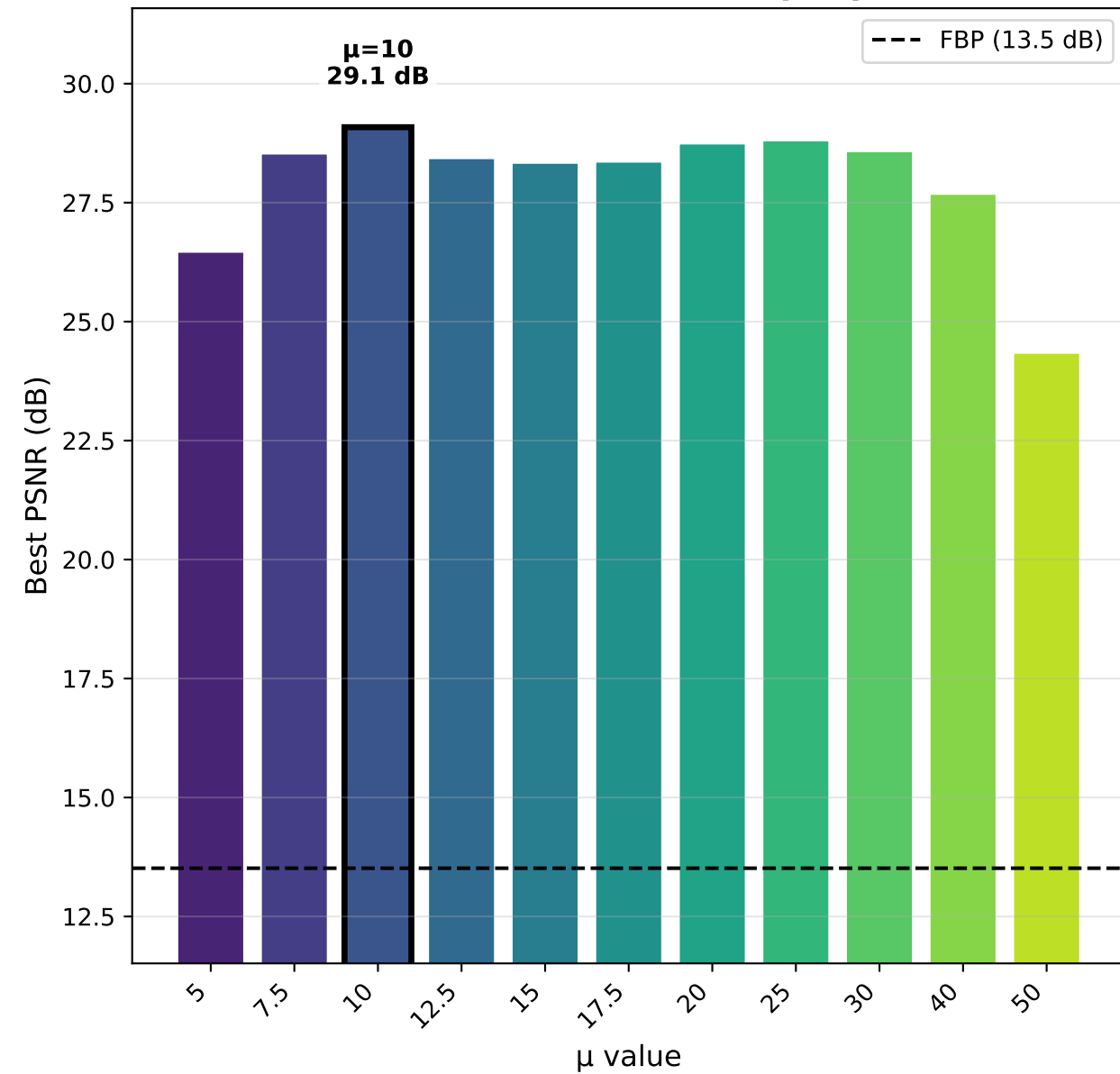
Best achievable PSNR per \mu
