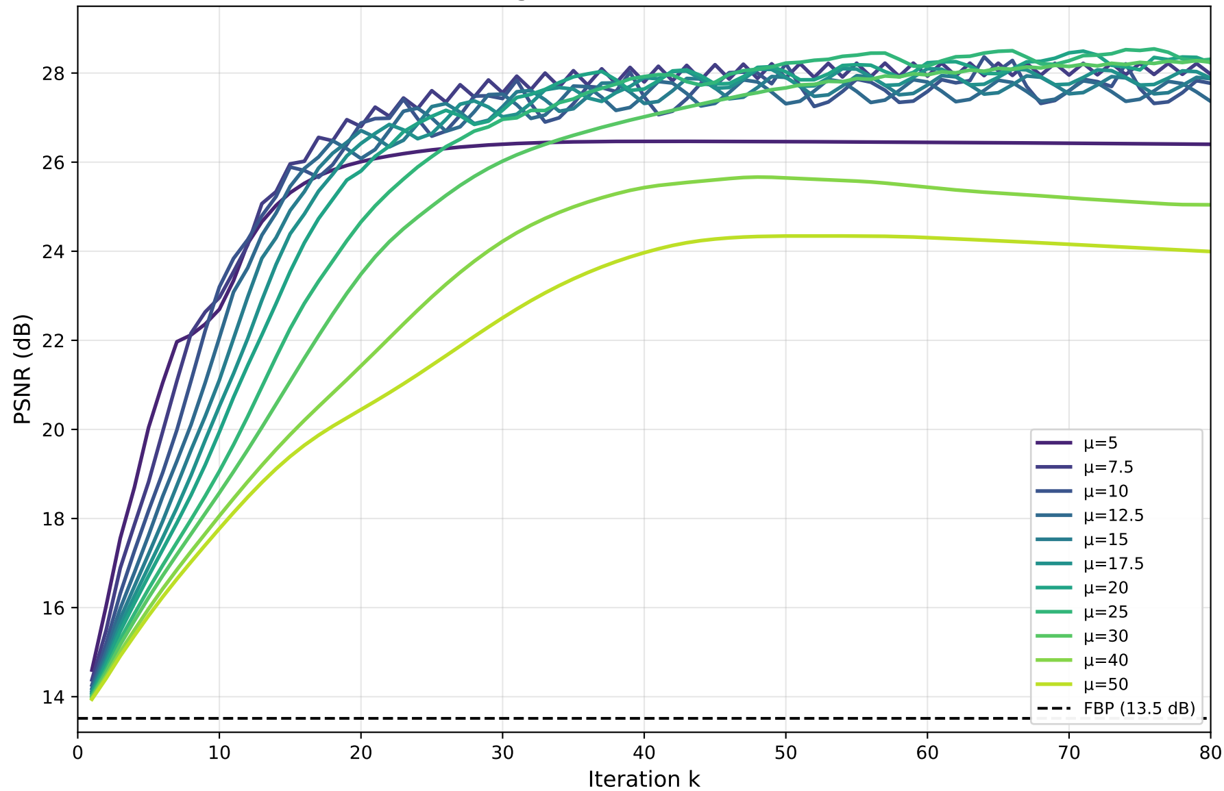
Convergence at \sigma=8 (CT-DRUNet)
