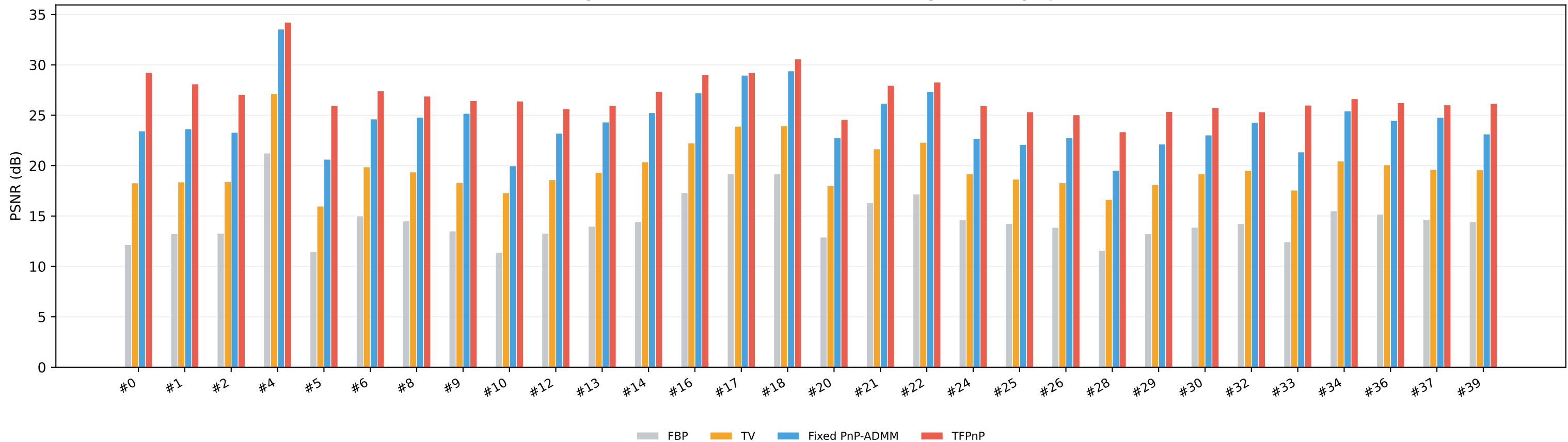
Per-Image PSNR at 5.0% Noise (30 of 40 images, evenly spaced)
