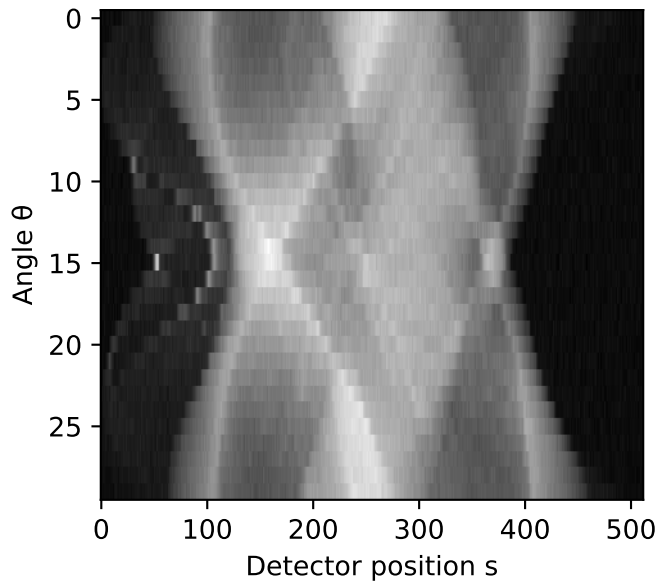
Sinogram y = Ax + \varepsilon 30 views, 5% noise
