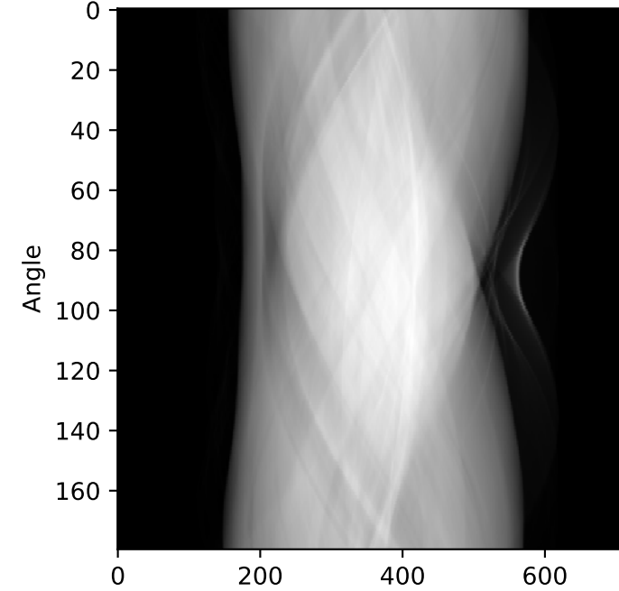
Sinogram — 180 views (dense)
