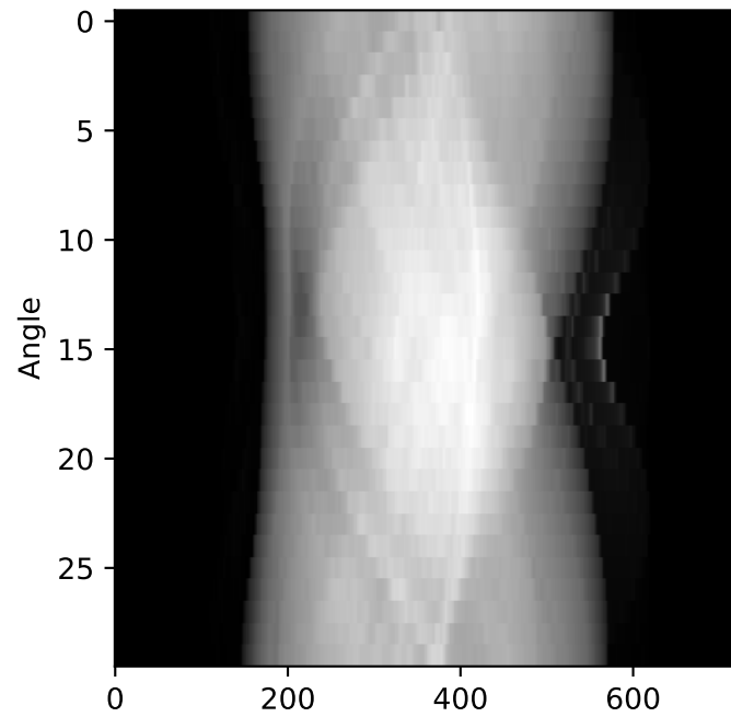
Sinogram — 30 views (sparse)
