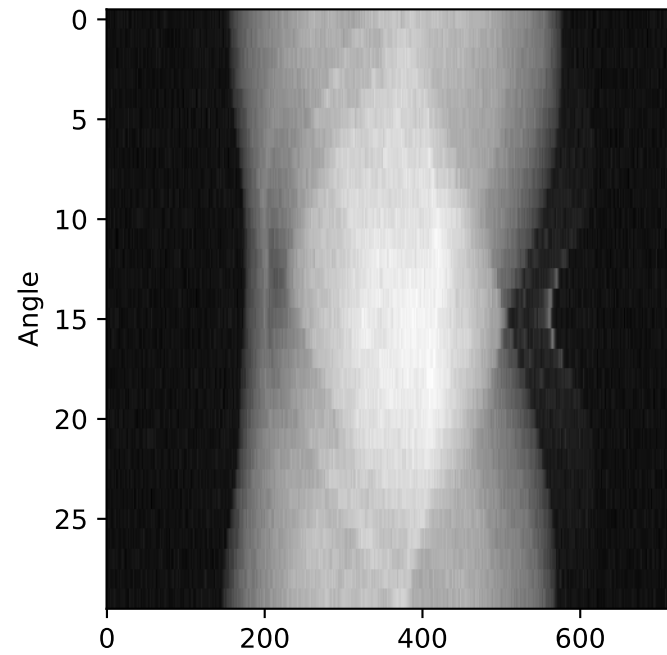
Sinogram — 30 views (noisy)
