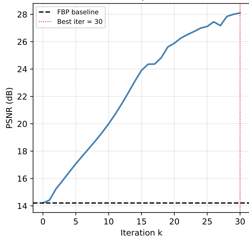
PnP-ADMM convergence ( \sigma=2.0 , \mu=20.0 )
