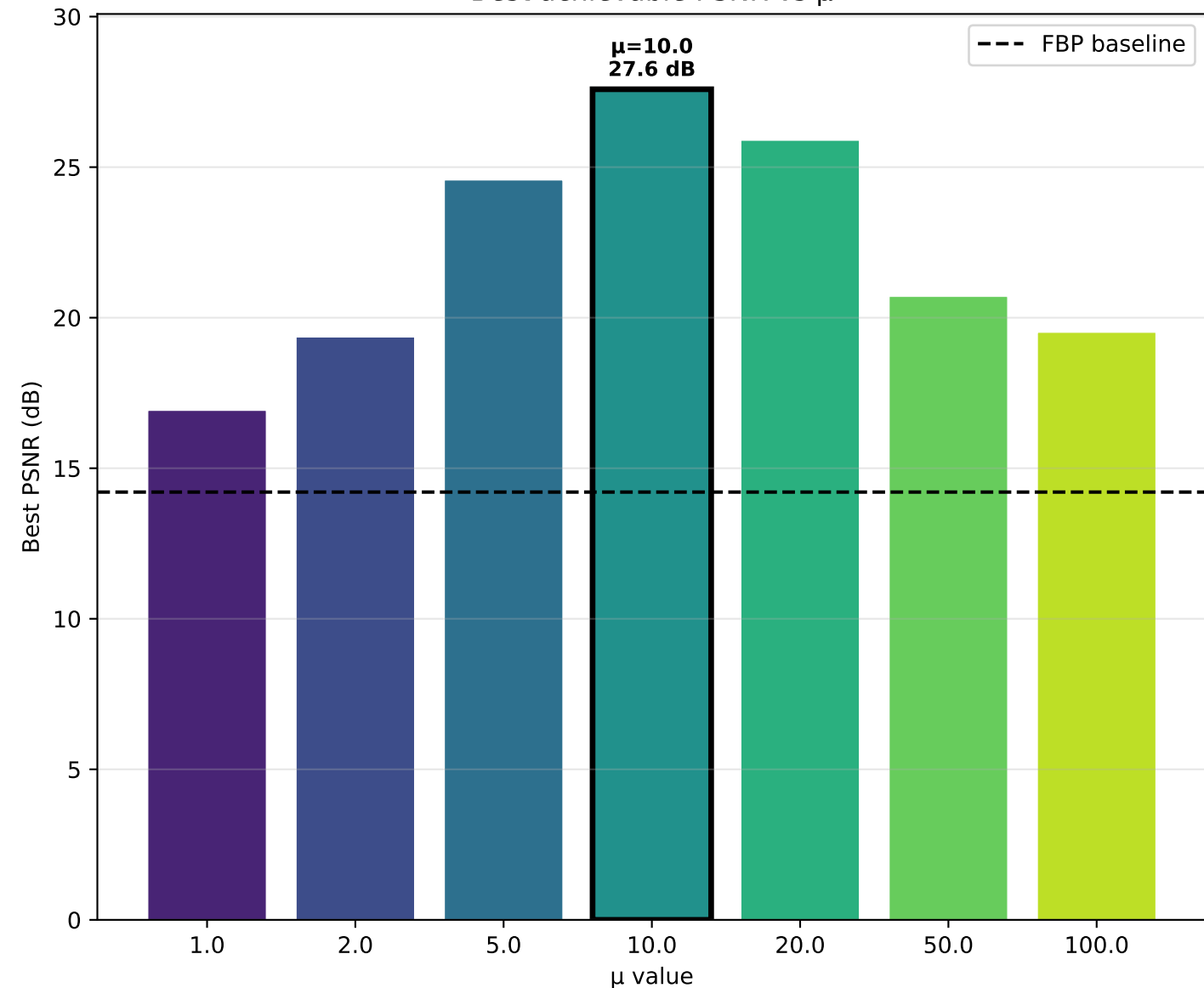
Best achievable PSNR vs \mu
