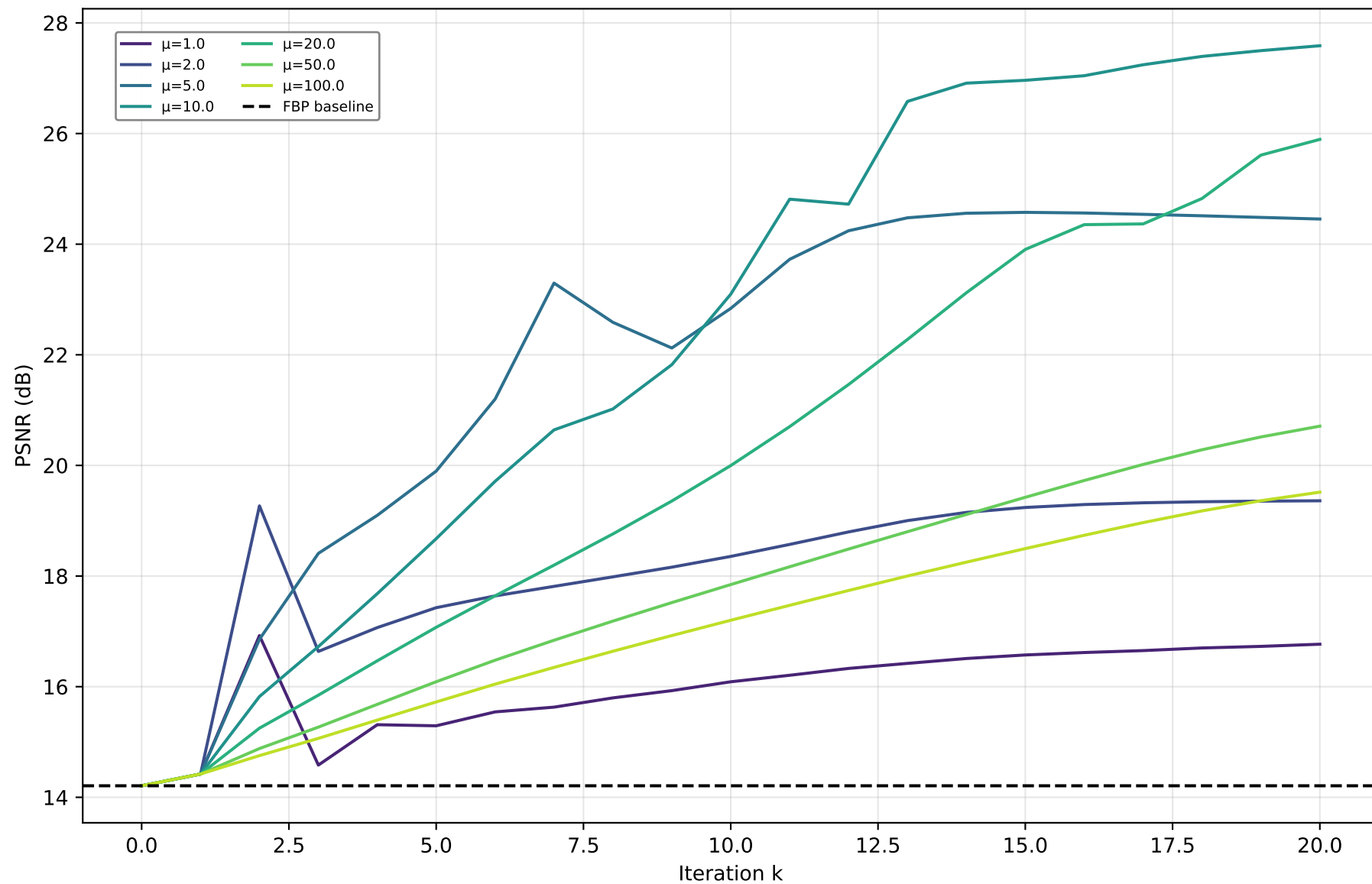
PSNR vs iteration for different \mu ( \sigma=2.0 fixed, DRUNet)
