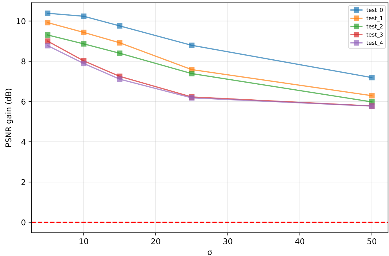
DRUNet PSNR improvement over noisy input
