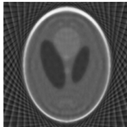
SIRT (30 views)
