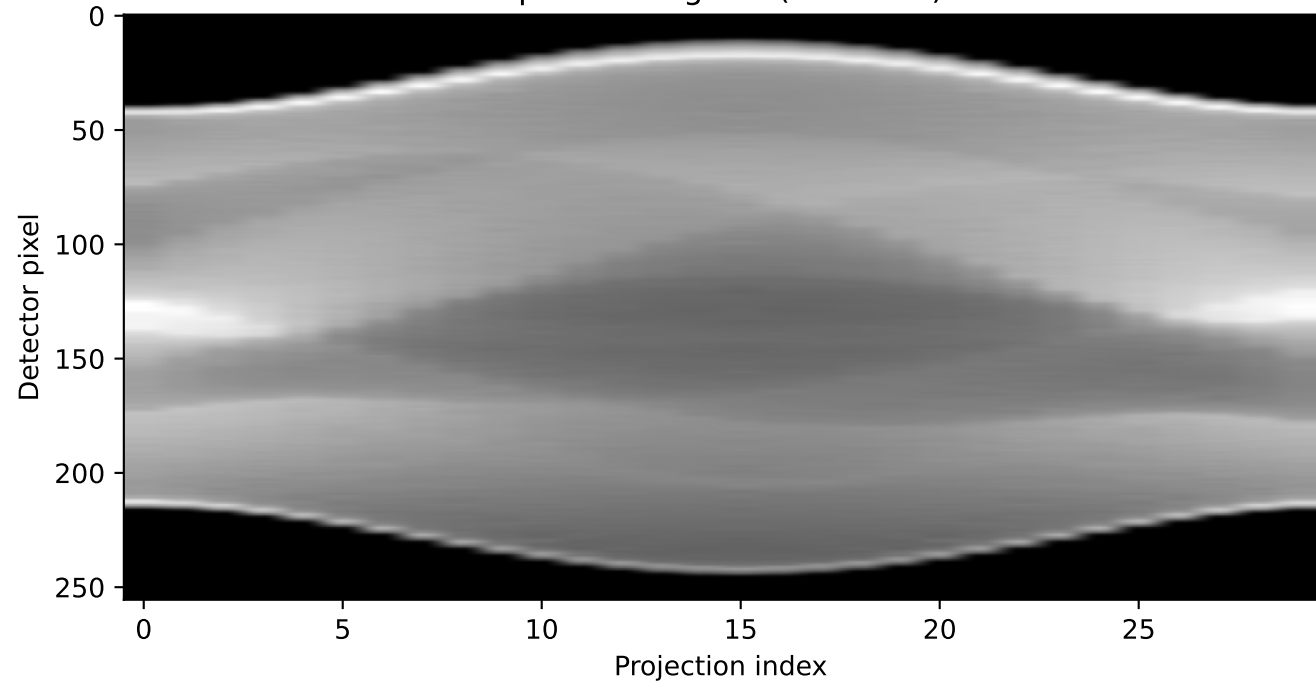
Sparse sinogram (30 views)
