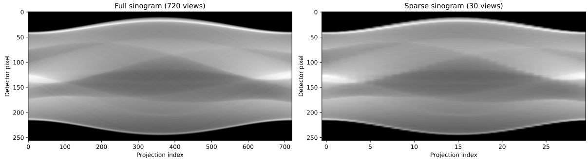
Figure 2.1: Sinogram comparison for the Shepp-Logan phantom. Left: full sinogram with 720 projection angles (the clinical standard). Right: sparse sinogram with only 30 angles, corresponding to a 24\times dosage reduction. The sparse sinogram contains the same sinusoidal structure but sampled at far fewer angular positions, leaving large gaps in the Radon domain.
