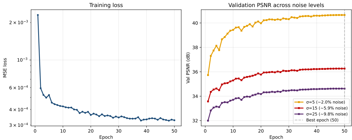
Figure 3.2: CT-DRUNet training curves. Left, MSE loss on the LIDC training split over 50 epochs. Right, validation PSNR at \sigma \in \{5, 15, 25\} . Best checkpoint by validation PSNR at \sigma = 15 .
