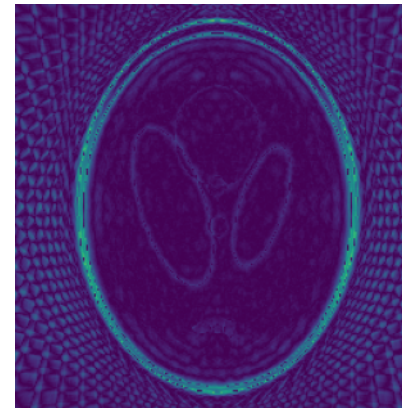
NAG_LS (30 views)
