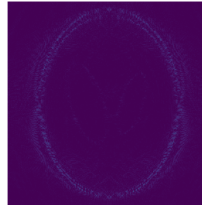
NAG_LS (720 views)
