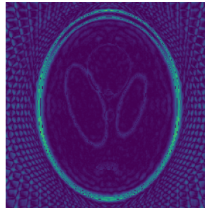
SIRT (30 views)
