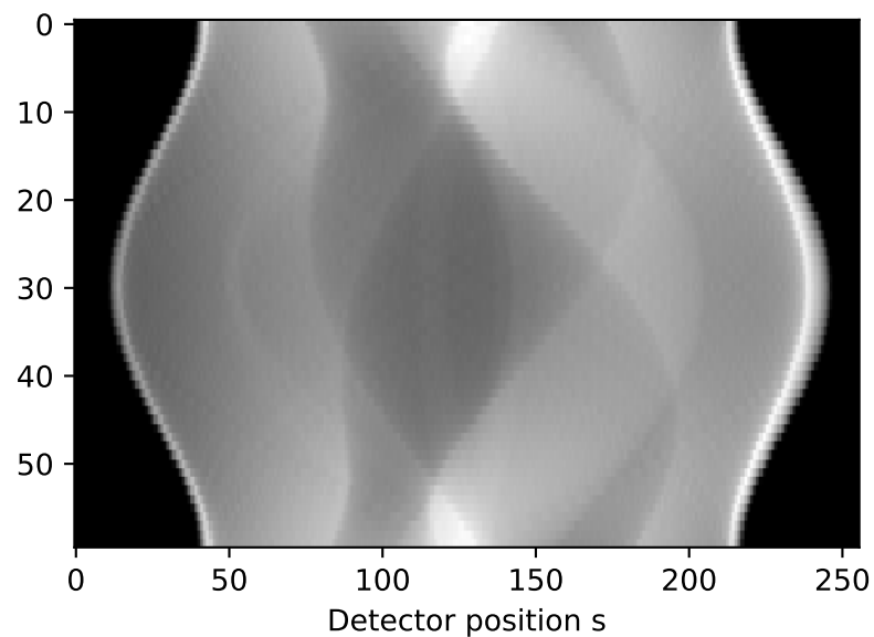
Mid sinogram (60 views)
