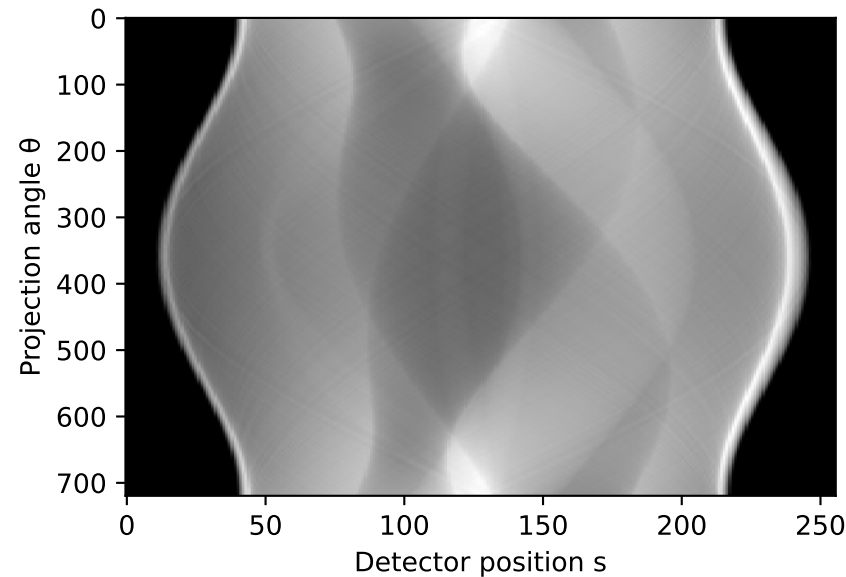
Full sinogram (720 views)
