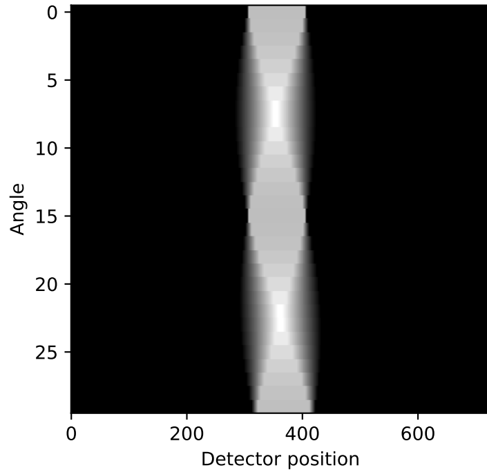
Sinogram Ax
