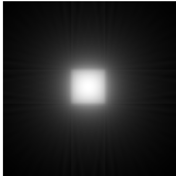
Backprojection A^T(Ax)
