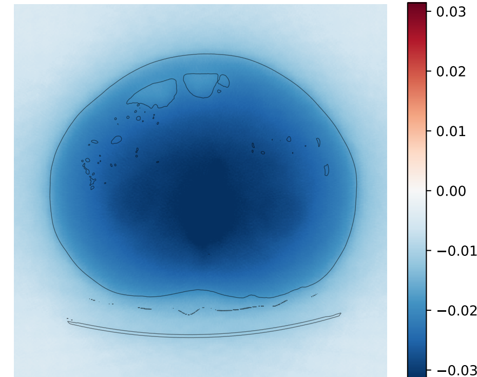
Dual variable u (accumulated disagreement, signed)
