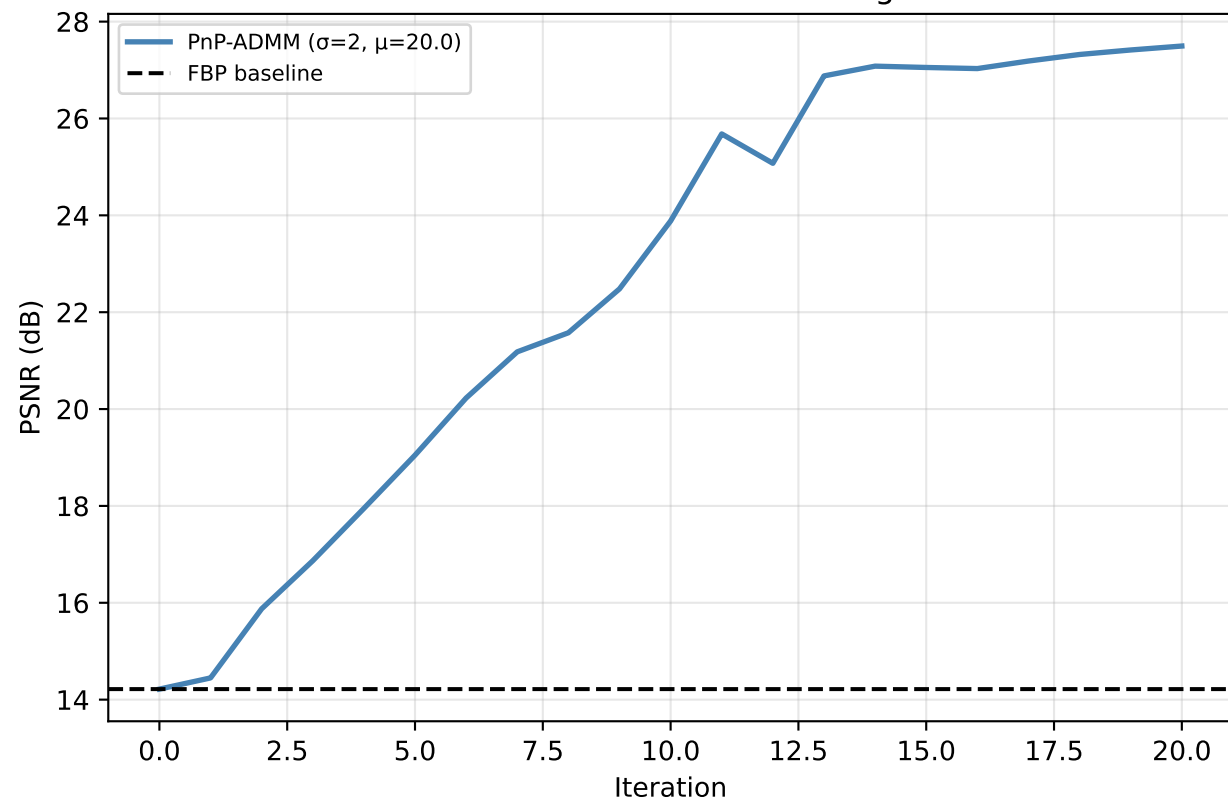
A: PnP-ADMM + DRUNet convergence
