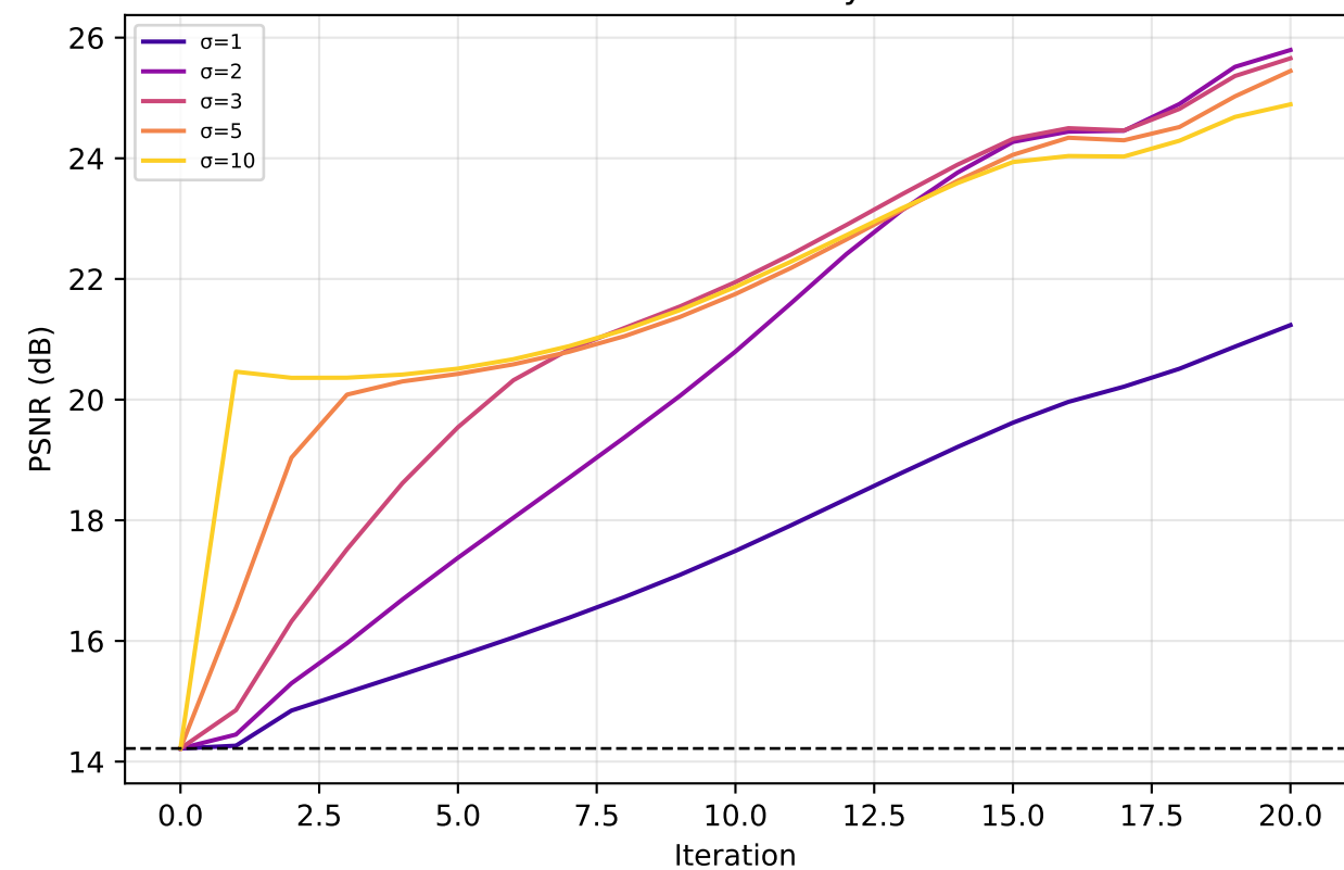
B: \sigma sensitivity
