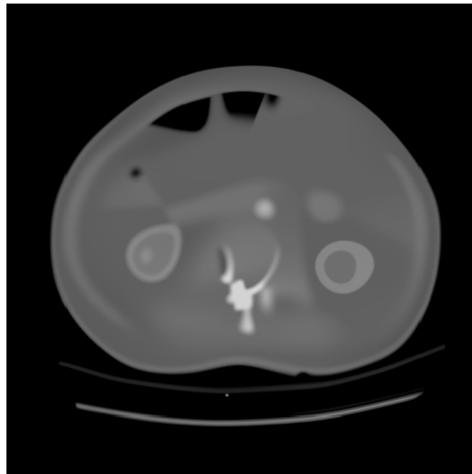
PnP-ADMM best (iter 186) PSNR = 31.1 dB
