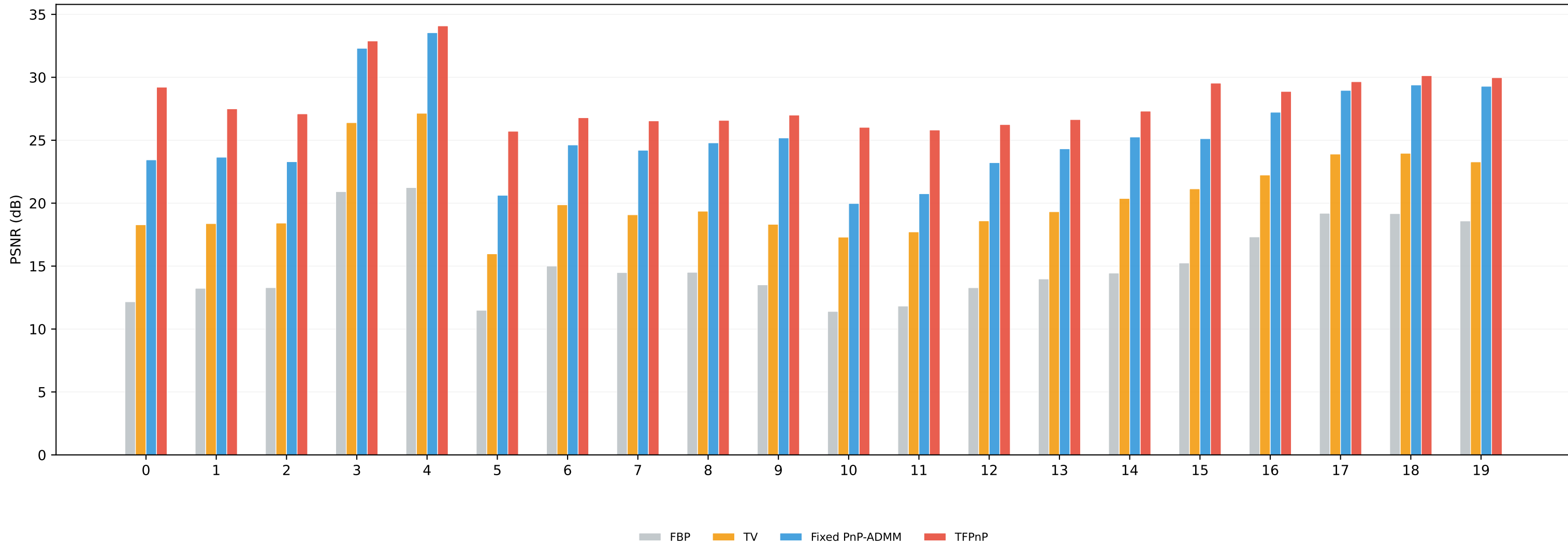
Per-Image PSNR at 5% Noise
