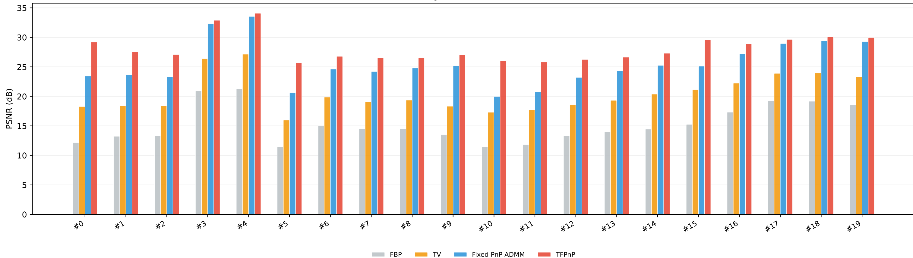
Per-Image PSNR at 5.0% Noise
