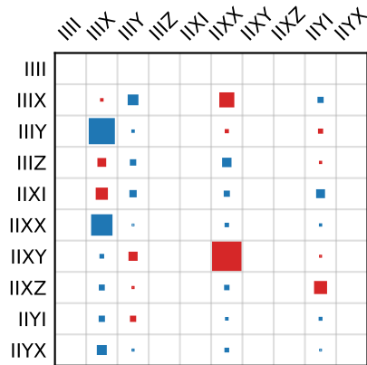
\text{id} - G U^{-1} (renormalized)
