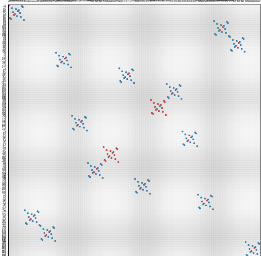
U (ideal gate)
