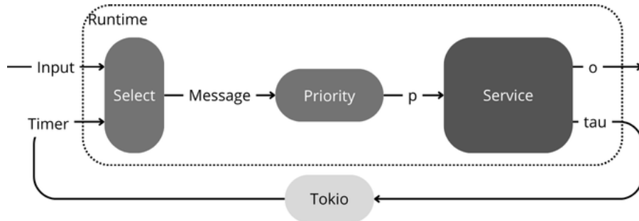
Figure 4.1: The execution of a service is handled by a runtime that processes import occurrences, propagates the corresponding equations within the service, and sends updated exports.
