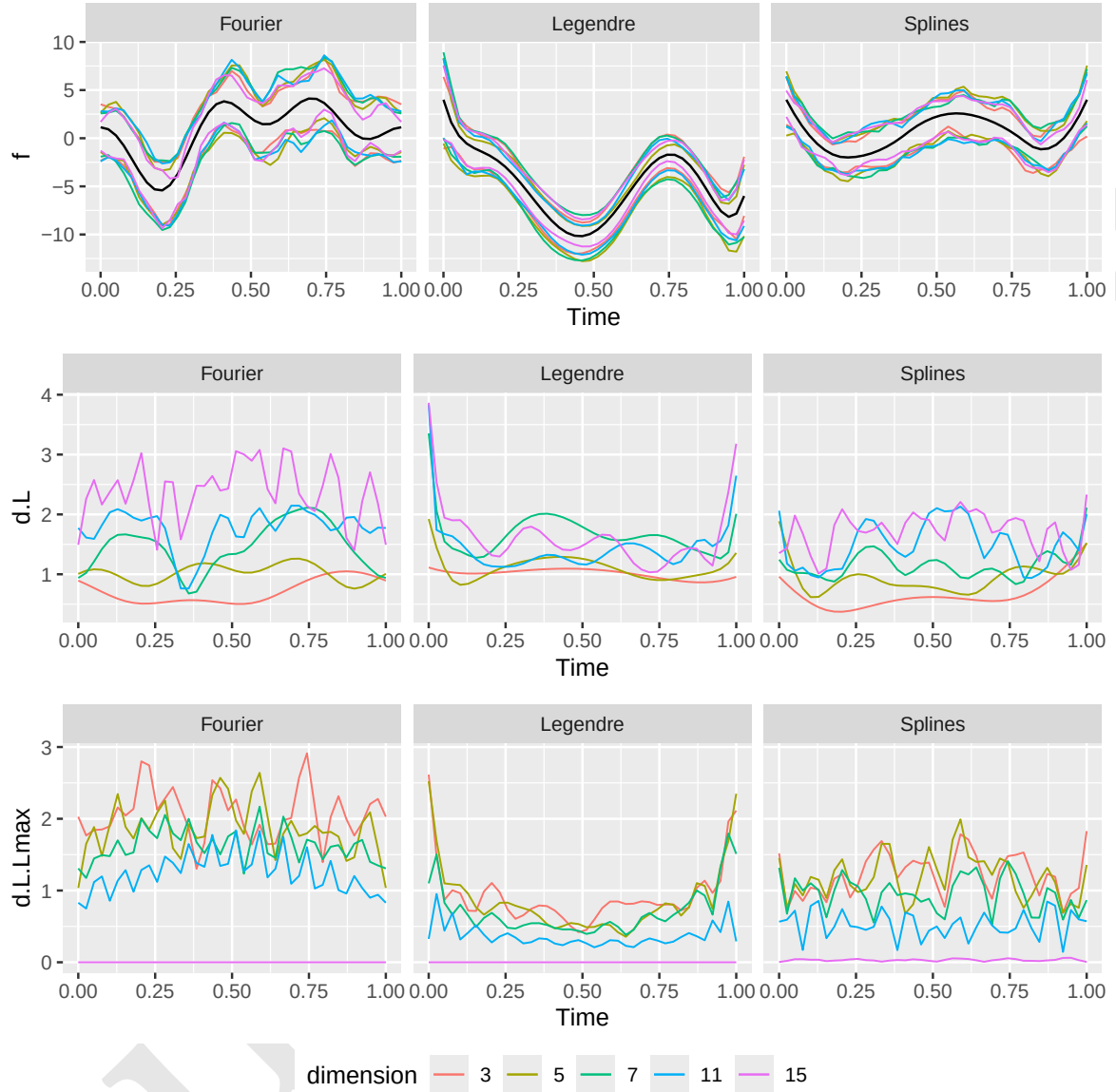
Figure 3: Visualization of confidence bands by correcting the bias. For a given dataset, we plot several confidence bands (top row), functions d.L (middle row) and d.L.L_{max} (bottom row). Bands and functions are estimated with Fourier (left column), Legendre (middle column) and Spline (right column) basis and several dimensions L (3, 5, 7, 11, 15), and L_{max} = 25 .
