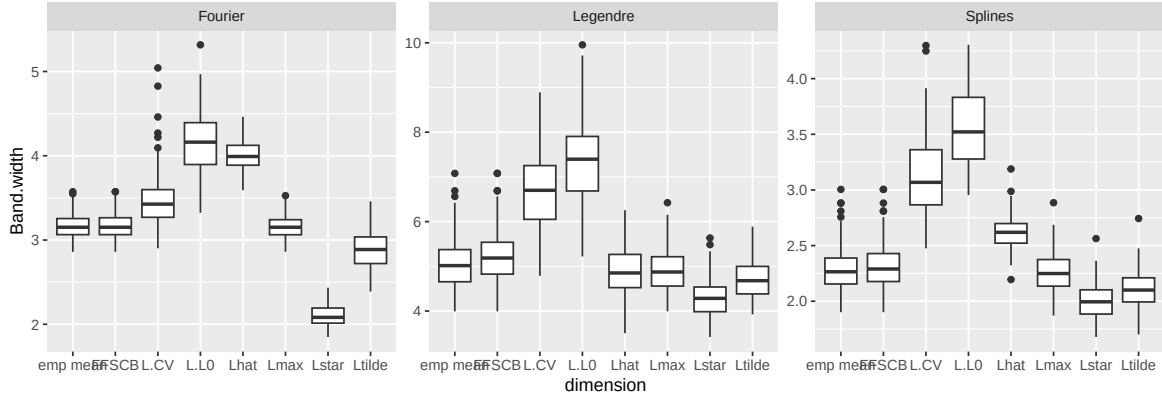
Figure 6: Illustrative example. We display within boxplots the confidence band's width over 100 repetitions for the dimension selected by the several criterion introduced in this paper, for Fourier (left), Legendre (middle) and Splines (right) basis.
