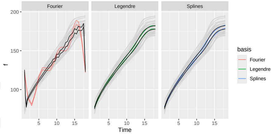
Figure 8: Real data analysis example. We display the confidence bands for Fourier (left), Legendre (middle) and Splines (right) basis on the Berkeley Growth Study data. Black curves correspond to the confidence bands with L_{max} , while colored one are the confidence bands with L_{tilde} .
