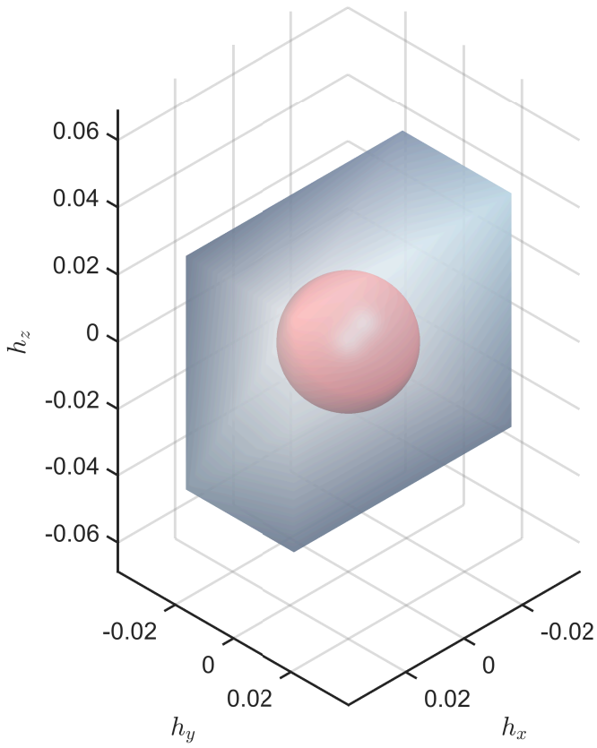
Angular Speed Envelope – 4 RWs Pyramid with 1 RW failure
