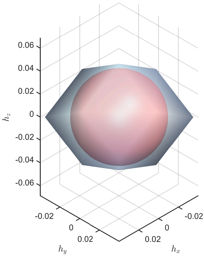
Angular Speed Envelope – 4 RWs Pyramid (open)
