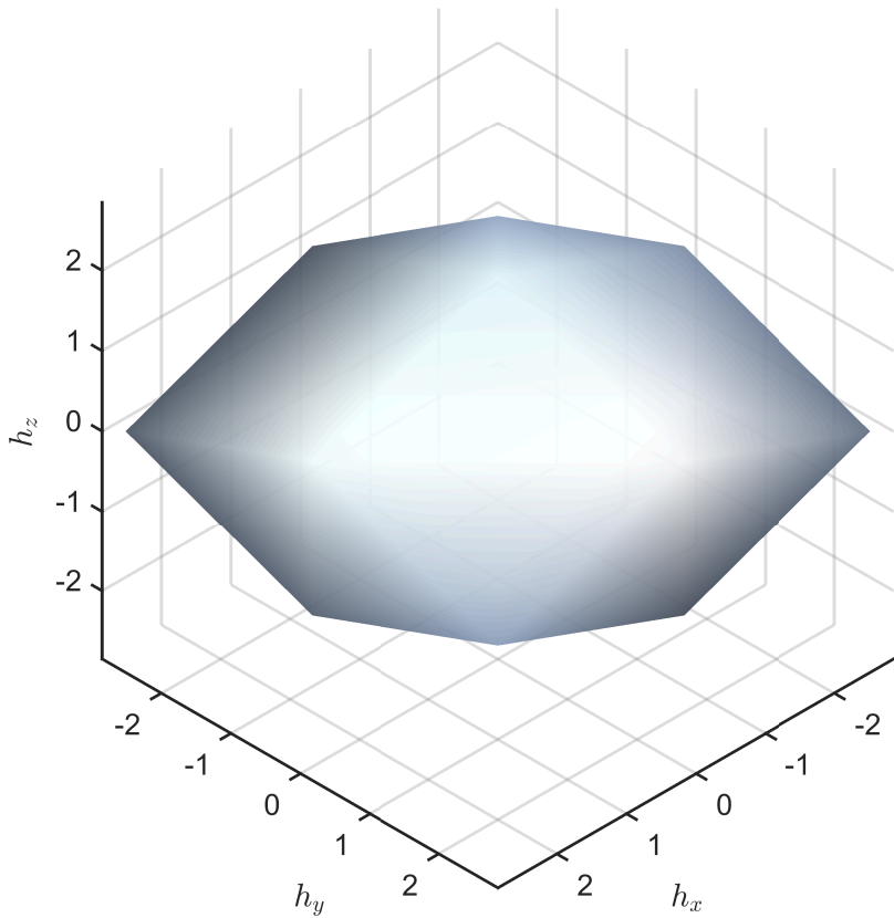
Angular Momentum Envelope – 4 RWs Pyramid
