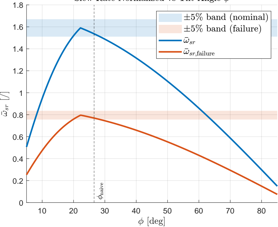
Slew Rate Normalized vs Tilt Angle \phi
