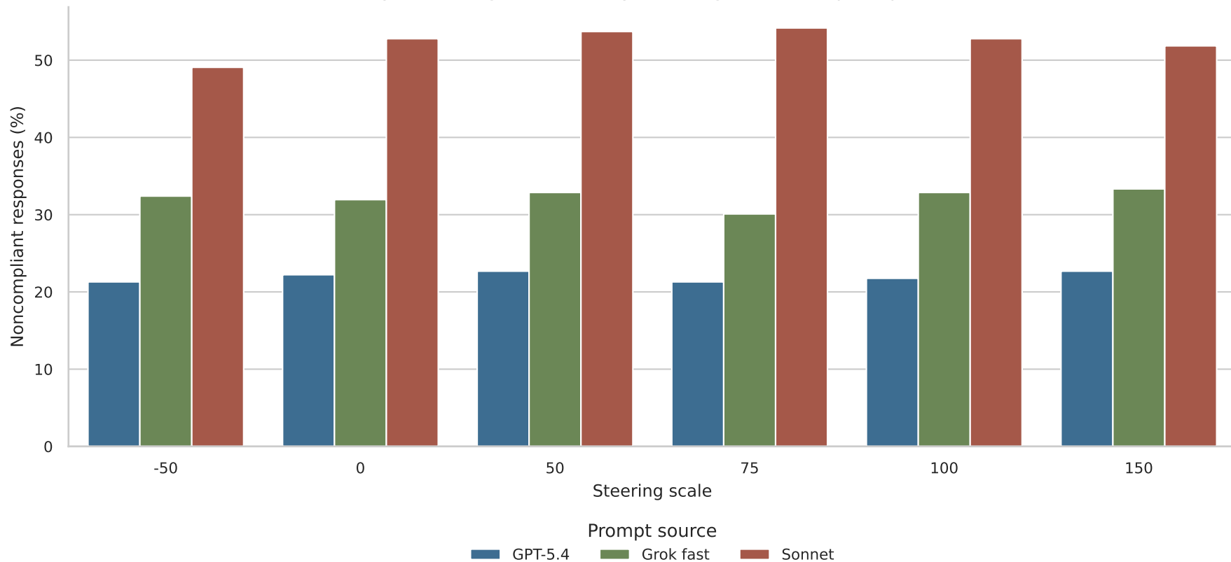
Exactly-two-integer failures by steering scale and prompt source
