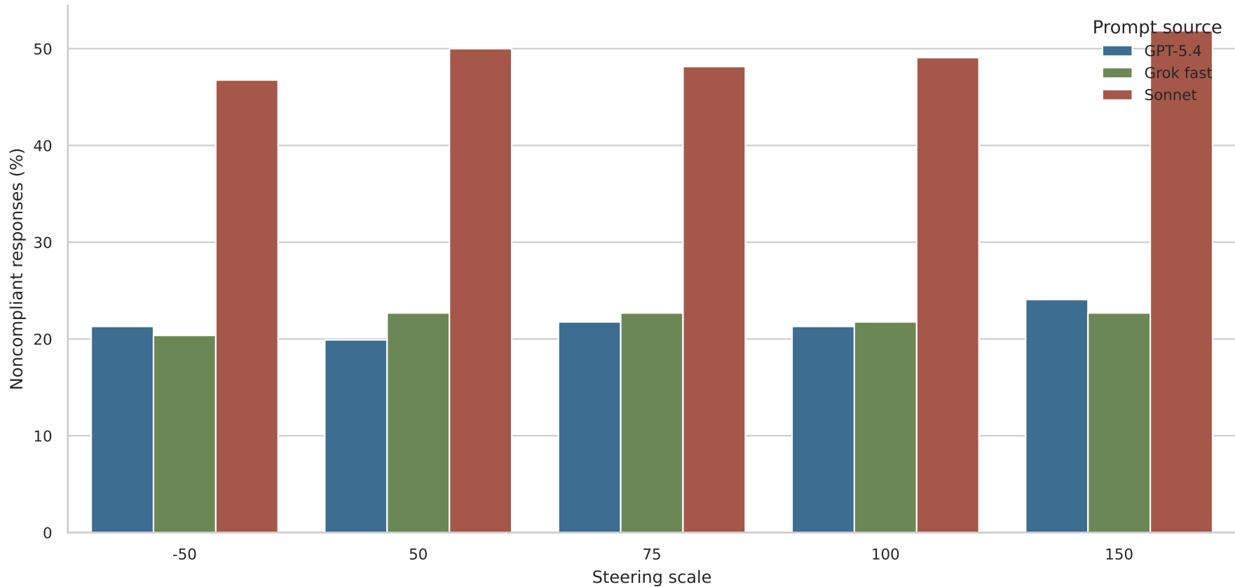
Exactly-two-integer failures by steering scale and prompt source
