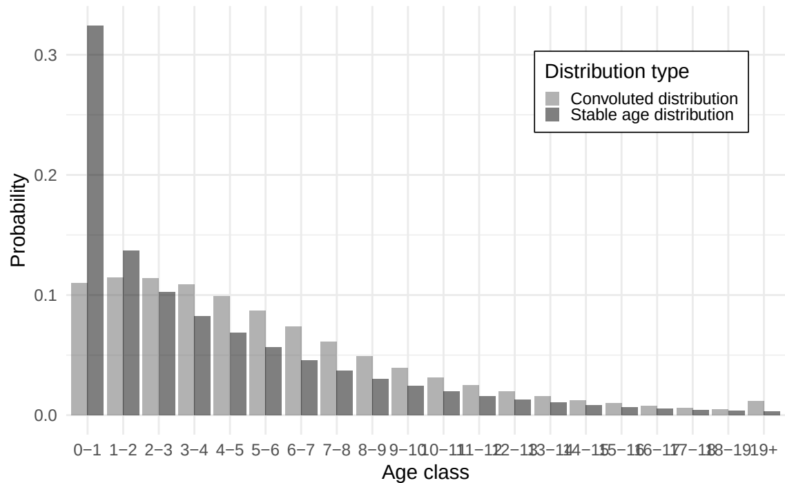
Stable age vs convoluted age distribution
