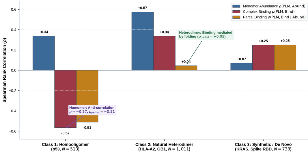
Figure 5: Evolutionary PPI stratification of interface variants ( N = 2,262 ) evaluated on ESMC-6B. In homooligomers (p53), sequence self-co-occurrence fails to rescue interface energetics, resulting in severe anti-correlation ( \rho = -0.565 , \rho_{\text{partial}} = -0.511 ). In natural heterodimers (HLA-A2, GB1), controlling for expression reduces partial binding correlation to \rho_{\text{partial}} = +0.045 . In synthetic binders and cross-species interfaces (KRAS, Spike RBD), uncoupled binding is weakly captured ( \rho_{\text{partial}} = +0.251 ).
