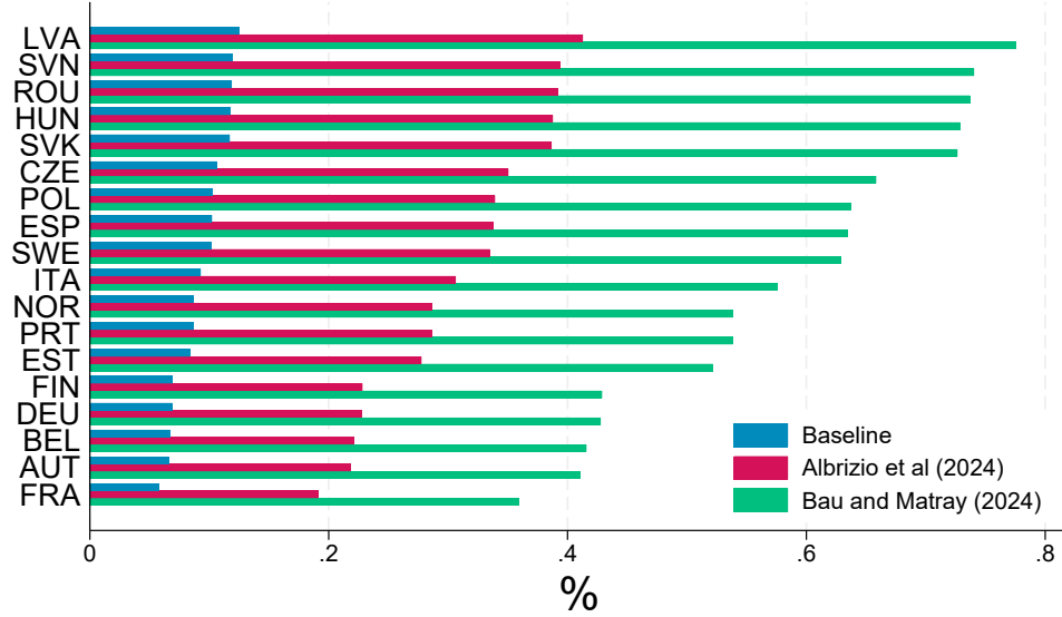
Figure D.1: \gamma estimates for different \nu .
