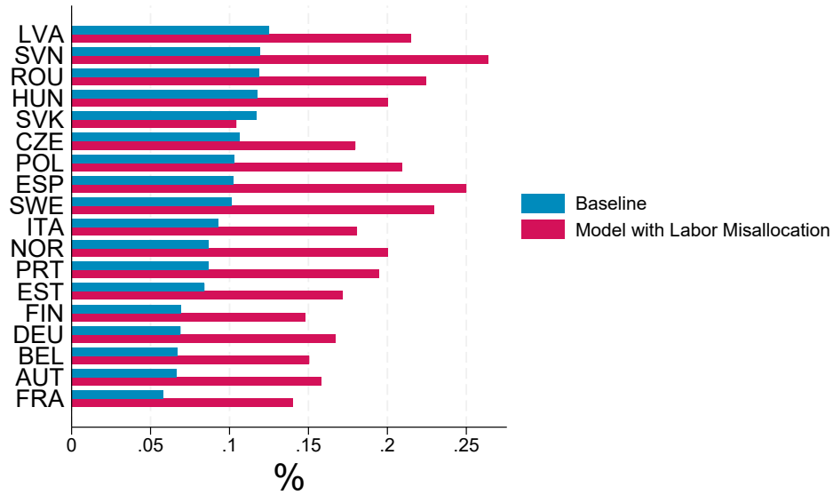
Figure D.1: Model with Labor Misallocation
