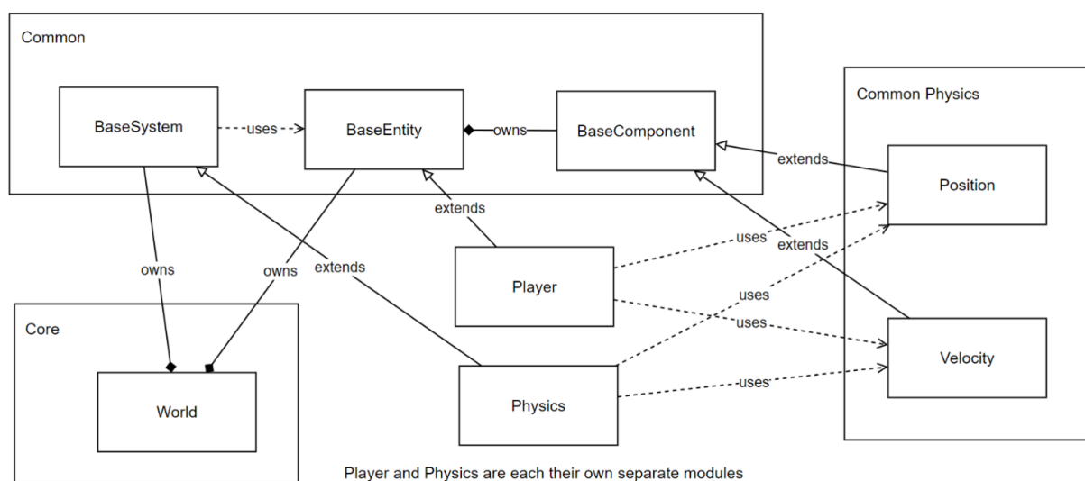
Figure 5: ECS Diagram.
