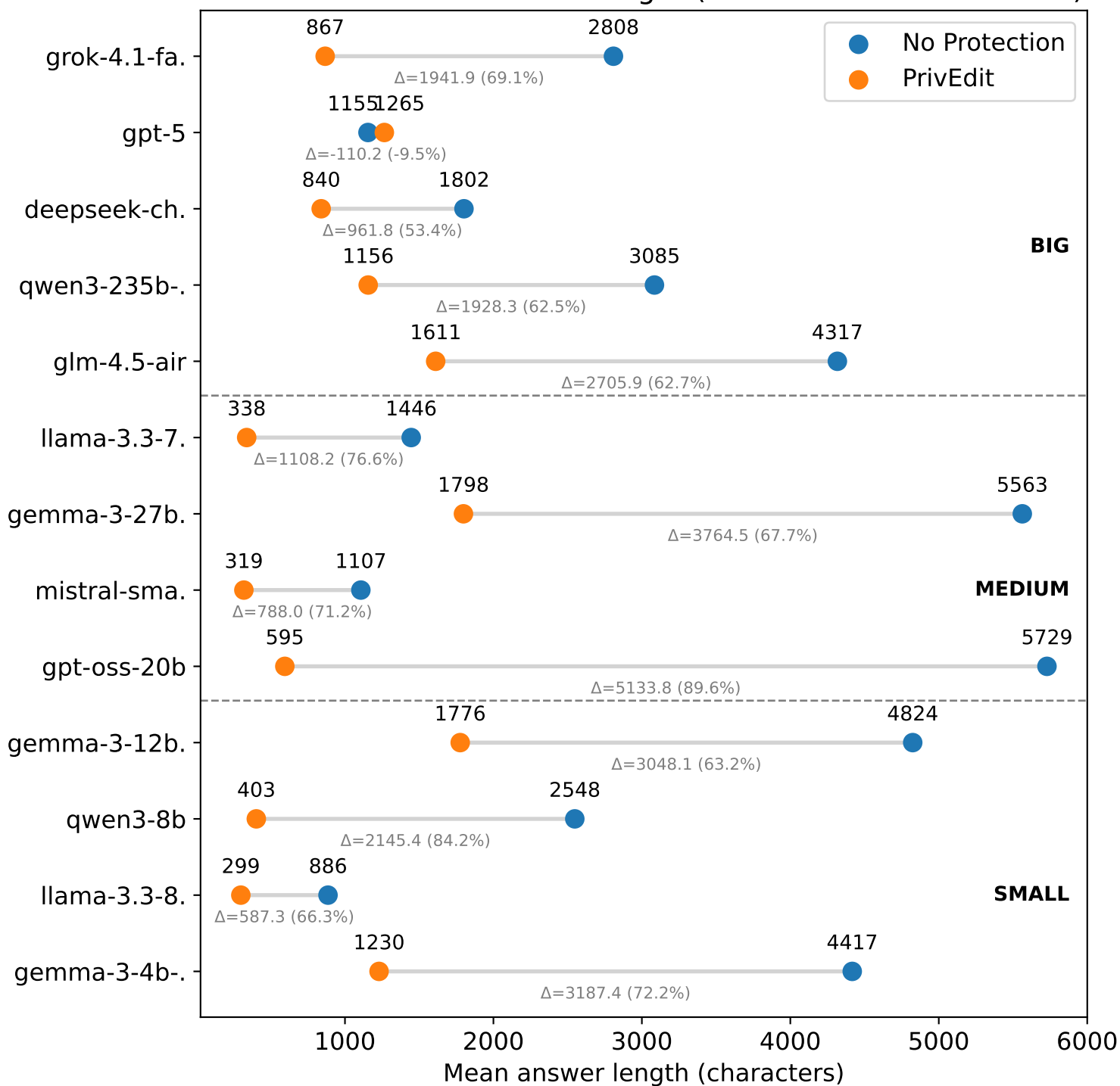
Decrease in mean answer length (No Protection vs. PrivEdit)
