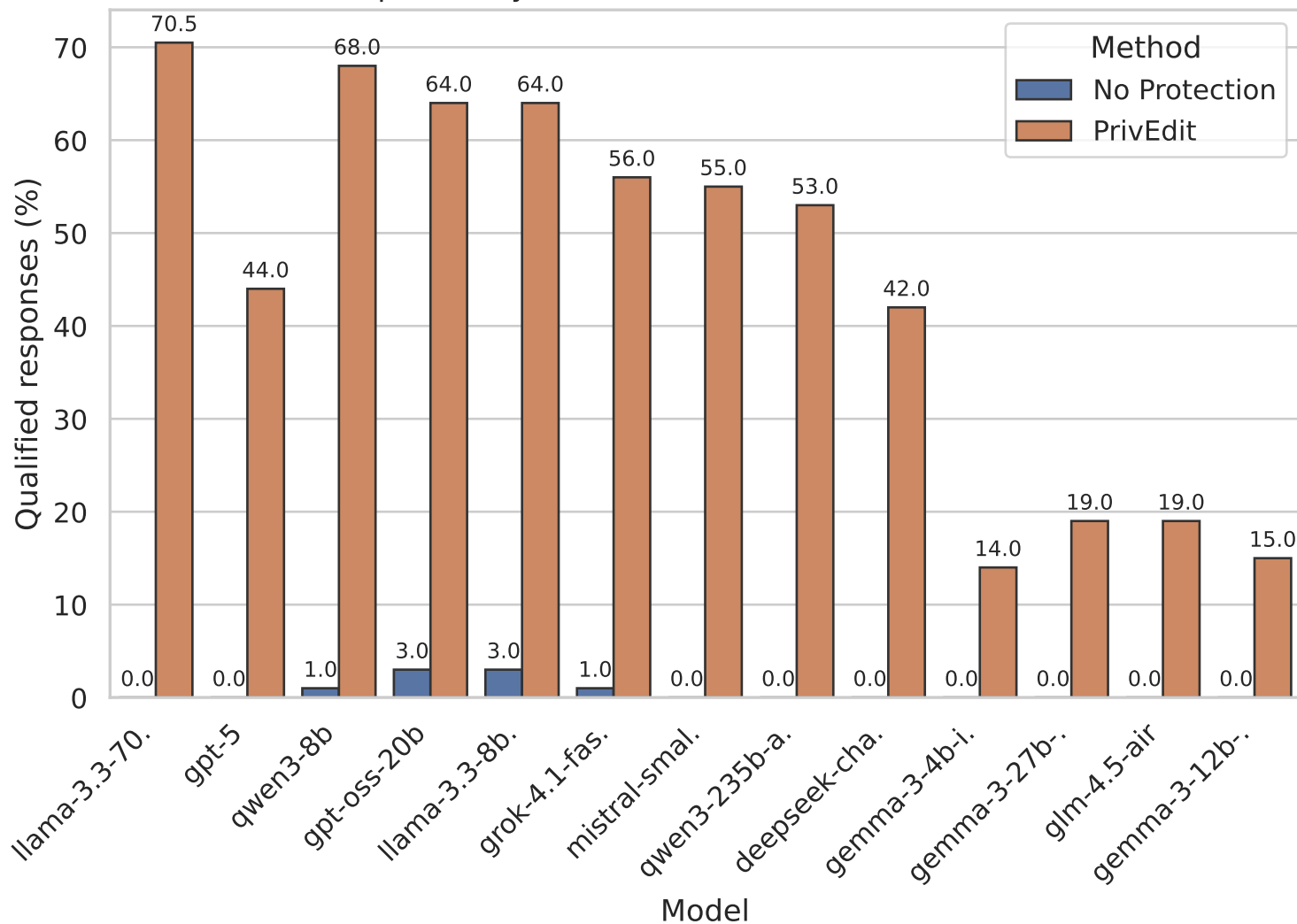
Qualified responses by model and method (No Protection vs PrivEdit)
