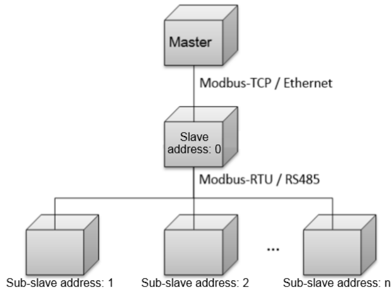
Figure 6-5 Communications address of the three-layer object structure
