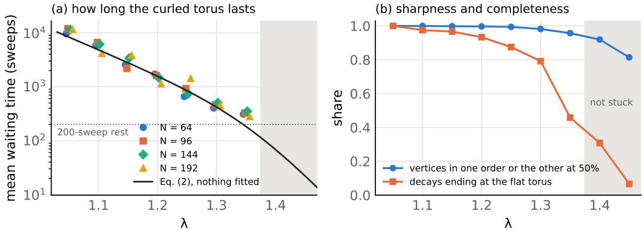
FIG. 3. The map along \lambda at g = 1.5 . (a) Mean waiting time where the torus is stuck, four sizes, with Eq. (2) (nothing fitted) and the 200-sweep rest; shaded, the \lambda at which it is not stuck. (b) Share of vertices in one order or the other at half conversion, and share of decays ending at the flat torus, pooled over sizes.
