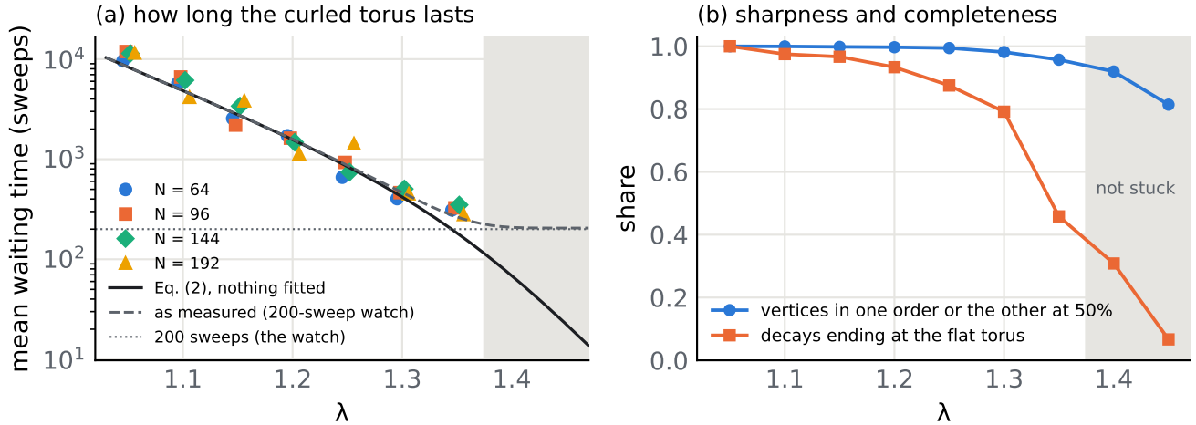
FIG. 3. The map along \lambda at g = 1.5 . (a) Mean waiting time where the torus is stuck, four sizes, with Eq. (2) (solid) and the same prediction as it would be recorded given the 200-sweep watch, 205 + \tau e^{-205/\tau} (dashed); both fitted to nothing. Shaded, the \lambda at which it is not stuck. (b) Share of vertices in one order or the other at half conversion, and share of decays ending at the flat torus, pooled over sizes.
