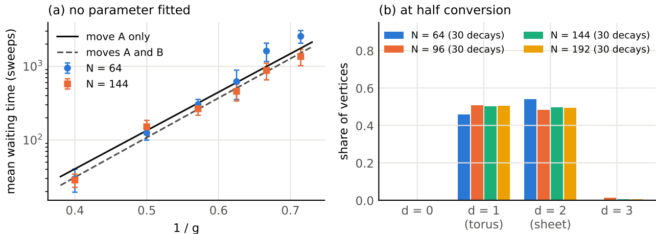
FIG. 1. (a) Mean waiting time of the perfect 4 \times L torus at \lambda = 1.25 against inverse coupling, sixteen runs per point, with Eq. (2) using move A only (solid) and moves A and B (dashed); nothing is fitted. (b) Share of vertices at each local dimension d when half the torus has converted, averaged over thirty decays per size.
