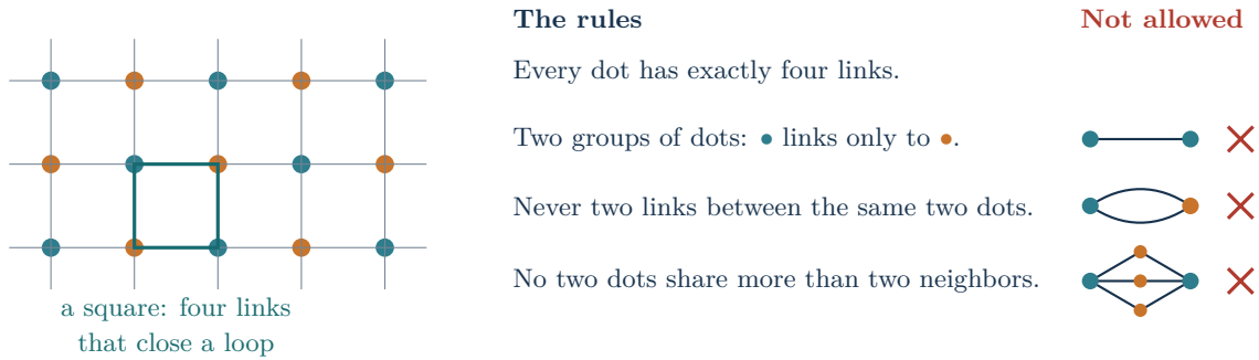
Figure 4. The whole model: dots, four links each, two groups, and the loops of four links called squares. There are no positions. Drawing the dots on a grid is a convenience; only the links are real.
