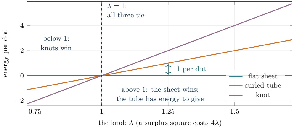
Figure 13. The ladder against the knob. EXACT Each line is one rung’s energy per dot as the surplus price changes. At \lambda = 1 , the published setting, the three rungs cost the same, so turning one into another releases nothing. Above 1 the sheet is lowest and the tube sits above it with a known amount to give: at \lambda = 1.25 , exactly one unit per dot. Below 1 the ladder flips and a sheet would gain by curling into knots, which is why the network breaks into knots when the surplus price is off.
