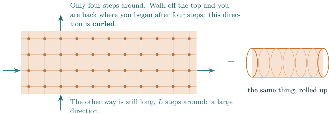
Figure 9. Curling one direction. EXACT Make one of the two ways around only four steps long. A grid four dots around and L dots along, wrapped both ways, is the 4 \times L torus. We call it the tube .
