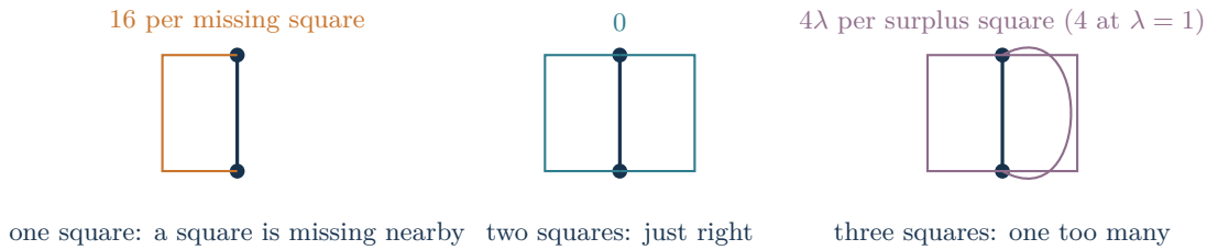
Figure 5. The price list, read link by link. EXACT The thick link carries one, two or three squares. Two is free. Fewer means a square is missing nearby, at 16 per missing square; a third is a surplus square, at 4\lambda , set by the knob. At \lambda = 1 the two prices make the energy a measure of the network's curvature; at \lambda = 0 a third square is free.
