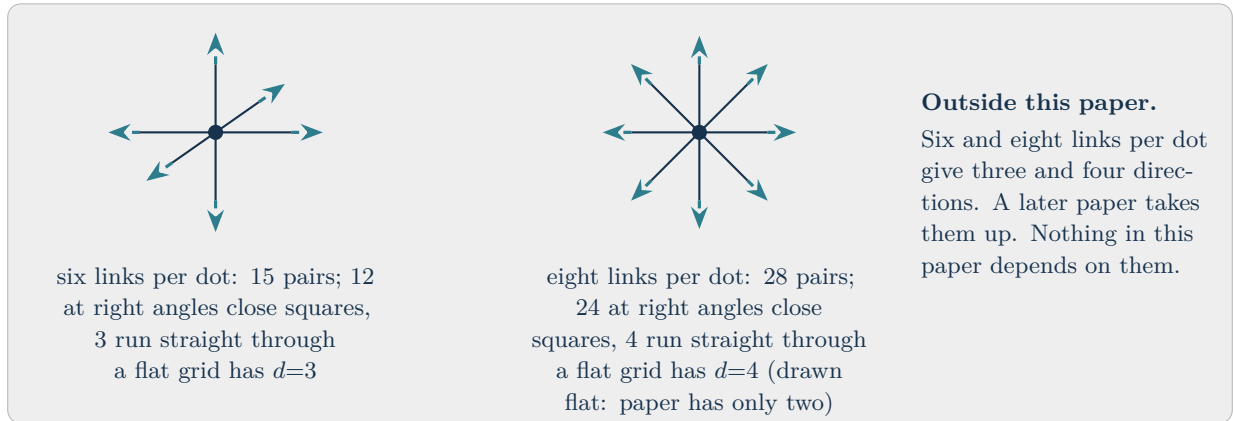
Figure 12. How many directions a dot has. EXACT Top: with four links per dot, the count d is the number of pairs of a dot's links that close no square, and it tells the flat sheet, the tube and the knot apart dot by dot. Grey box, outside this paper: the same count with six or eight links per dot allows three or four large directions, the subject of a later paper. The count is a signature, not a certified geometry: Chapter 6 says what it can and cannot vouch for.
