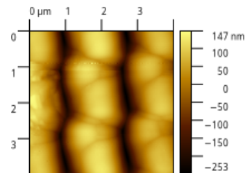
Figura 3: Scansione 4 \times 4 \mu\text{m}^2 .
