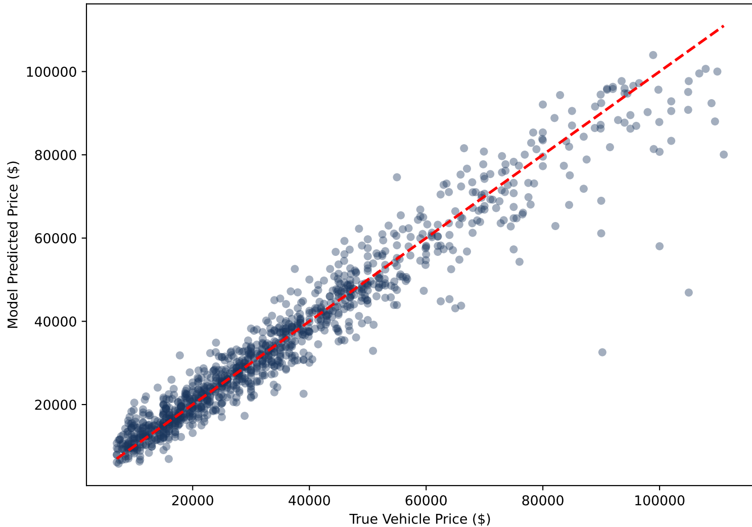
Actual Prices vs. True Champion Ensemble Predictions ( R^2 = 0.9306 )
